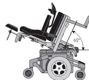
Figure 1: Tilt System
